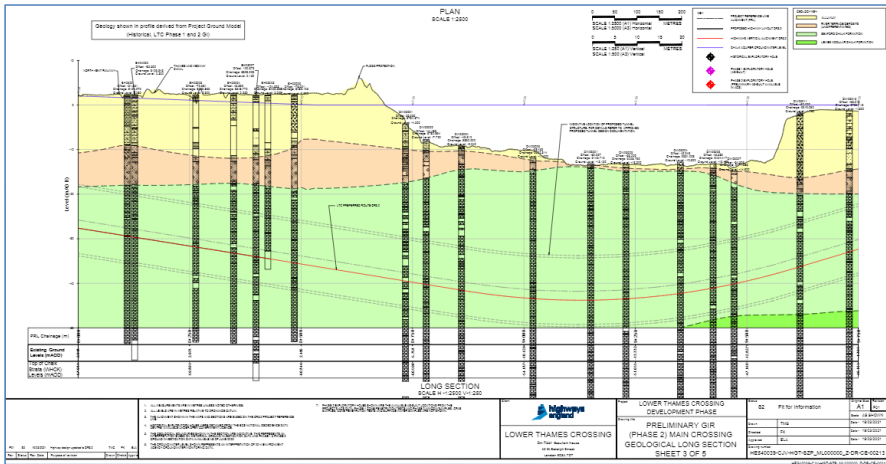
Plate 8.1 Geological interpretation long section across the river along the tunnel alignment
